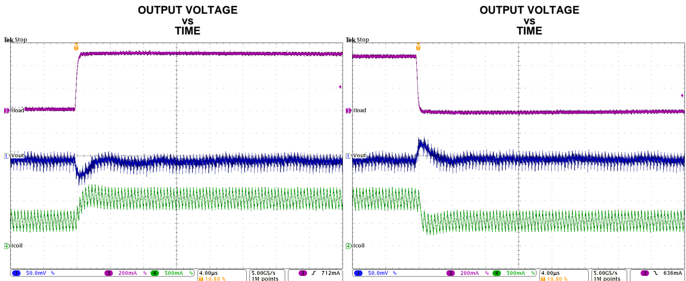
Figure 31. Line Transient Response of Figure 30, rising edge
